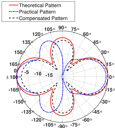
FIGURE 17. Normalized beam pattern with the combined near UT-based analog beamforming weights using staggered 3D UCA, generated by MOM/EM simulation.
