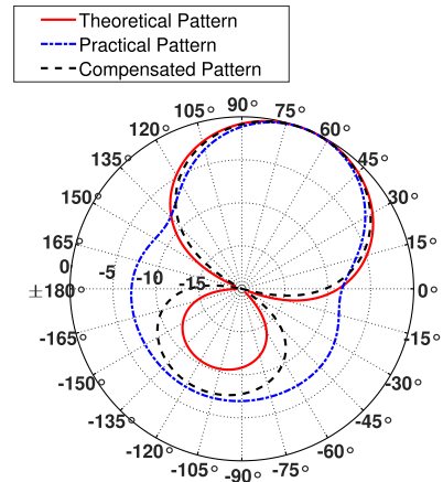
FIGURE 11. Normalized beam pattern with nearest UT-based analog beamformer \mathbf{v} = \mathbf{a}(\phi_1) , employing UCA with N = 8 and r = 0.25\lambda .
