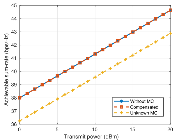
FIGURE 13. Total achievable sum-rate of downlink NOMA using UCA with N = 8 , r = 0.25\lambda and \phi = [68^\circ, 60^\circ, 50^\circ, 80^\circ] .
