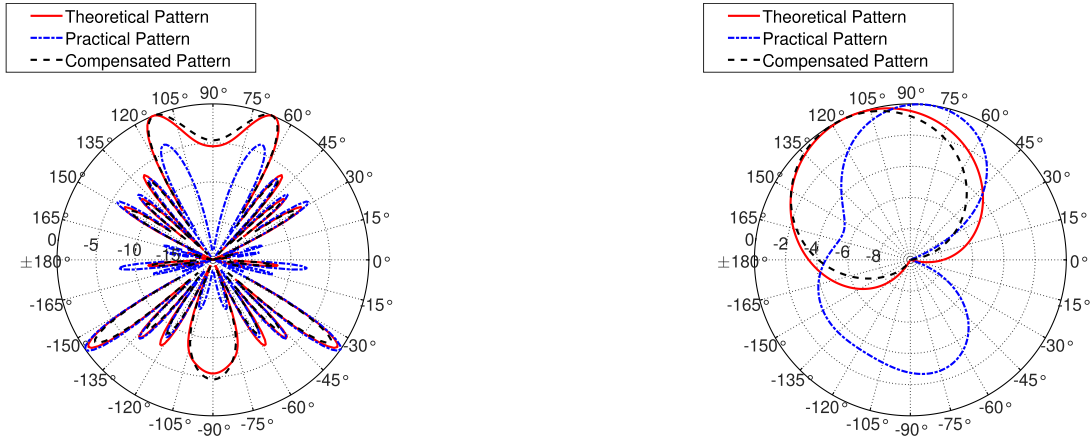
FIGURE 4. Normalized YZ-plane pattern with nearest UT-based beamformer, employing ULA with N = 16 and d = 0.5\lambda , MOM/EM simulation.
