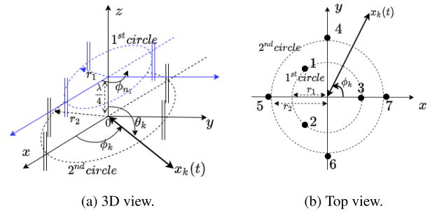
FIGURE 3. Uniform circular array geometry with staggered UCA at z = \lambda/4 : (a) 3D view, (b) Top view in XY -plane.
