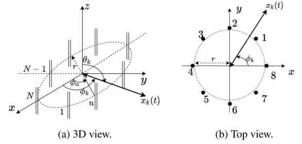
FIGURE 2. Uniform circular array geometry: (a) 3D view, (b) Top view in XY -plane.
