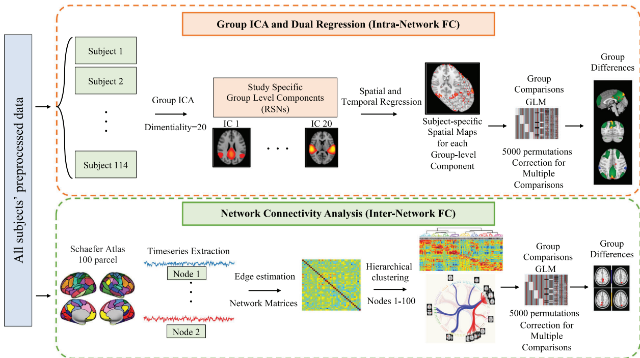
FIGURE 1 Analysis pipeline.
