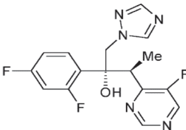
Figure 1. Chemical structure of voriconazole molecule
