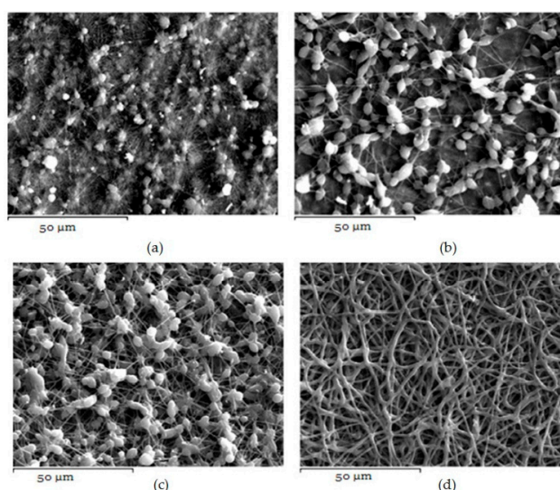
Figure 2. PCL fibers prepared using different concentrations of PCL in DCM/DMF-70/30 v/v mixture. (a) 5%; (b) 10%; (c) 15%; and (d) 20% w/v .
