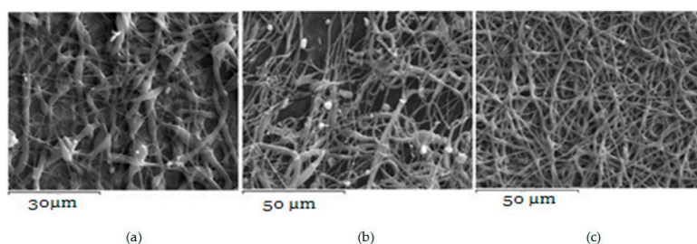
Figure 1. Poly( \epsilon -caprolactone) (PCL) fibers produced by a 20 wt % PCL solution using as solvent: (a) DCM; (b) DCM/Acetone (70/30 v/v ); and (c) DCM/DMF (70/30 v/v ).
