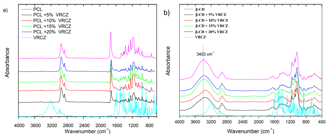
Figure 8. (a) FT-IR spectra of PCL fibers containing VRCZ and (b) FT-IR spectra of VRCZ inclusion complexes.
