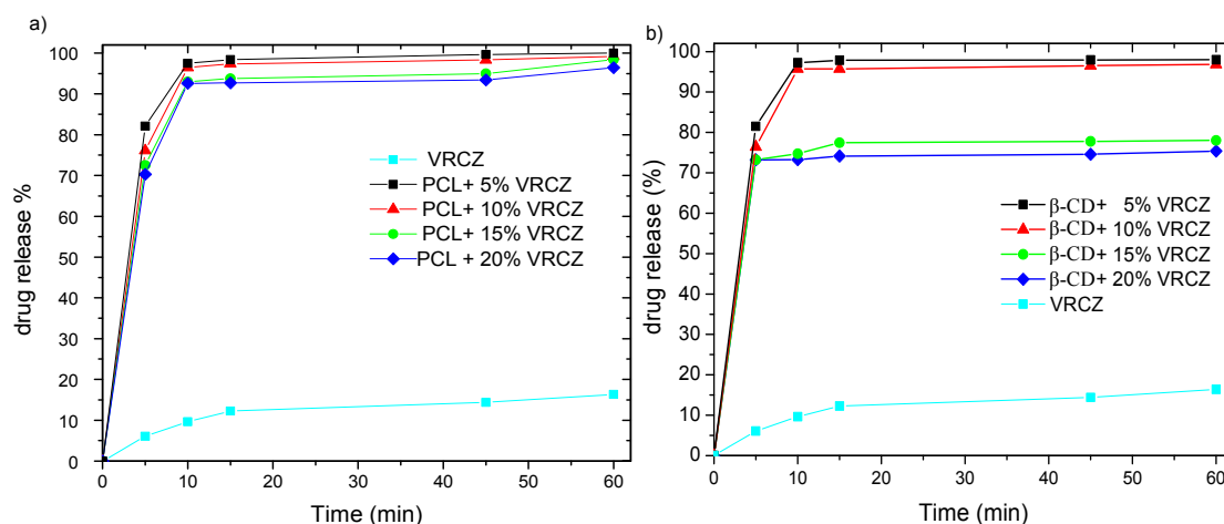
Figure 9. (a) In vitro release studies of PCL fibers containing VRCZ and (b) in vitro release studies of VRCZ inclusion complexes.
