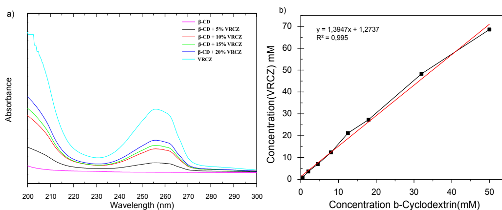
Figure 5. (a) UV-VIS spectroscopy and (b) phase solubility studies of \beta -CD/VRCZ inclusion complexes. (Red line is associated as trend line).
