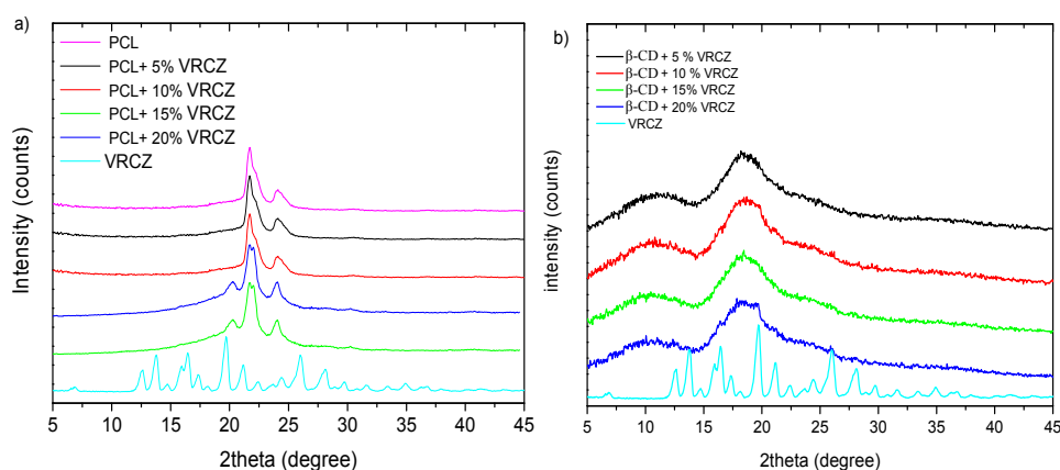
Figure 7. X-ray diffraction patterns of (a) PCL fibers containing VRCZ; and (b) VRCZ inclusion complexes with \beta -CD.
