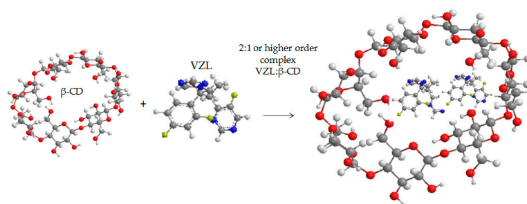
Figure 6. Complexation between VRCZ drug and \beta -CD.
