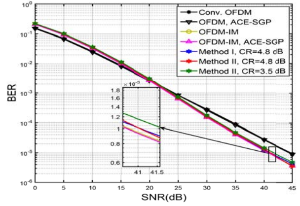
Fig. 6. The BER curves for the comparison of the proposed methods.
