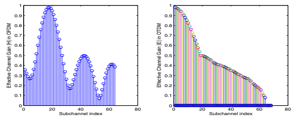
Fig. 3. Comparison between the effective channel transform responses of OFDM (left shape) and OTDM (right shape).
