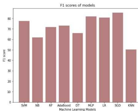
Fig. 8: Comparison of f1 scores of all models with bar plotting.
