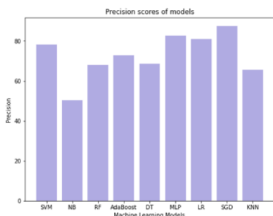
Fig. 6: Comparison of precision scores of all models with bar plotting.
