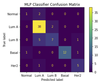
Fig. 3: MLP Classifier model confusion matrix.
