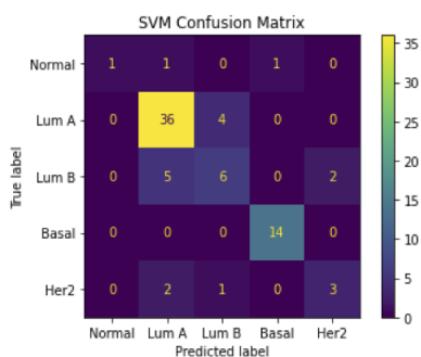
Fig. 4: SVM model confusion matrix.
