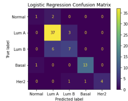
Fig. 2: Logistic Regression model confusion matrix.
