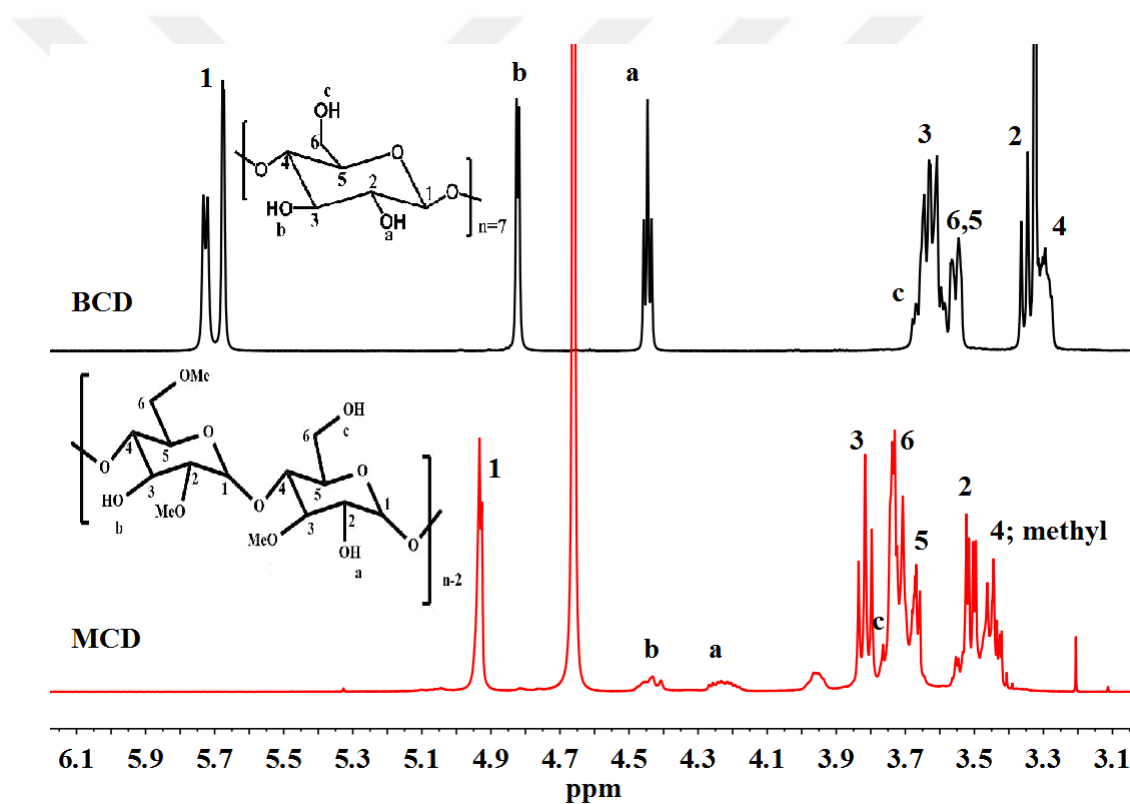
Figure 4.3: ^1\text{H} NMR spectrum of BCD and MCD. A clear peak shift and a decrease in the intensities of a, b, and c can be seen.
