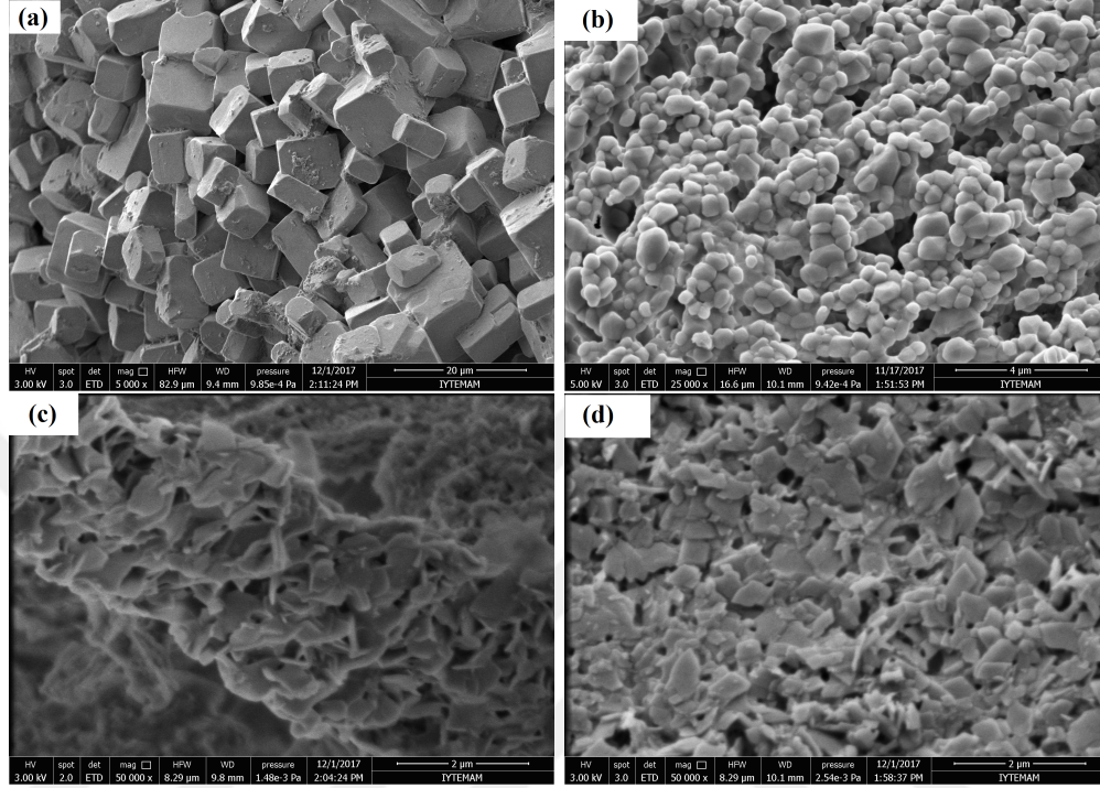
Figure 4.16: SEM images of freeze dried MIC at a concentration of 0.1 mg/mL and 1.0 mg/mL in PBS and water. (a) 0.1 mg/mL in PBS, (b) 1.0 mg/mL in PBS, (c) 0.1 mg/mL in water, and (d) 1.0 mg/mL in water.
