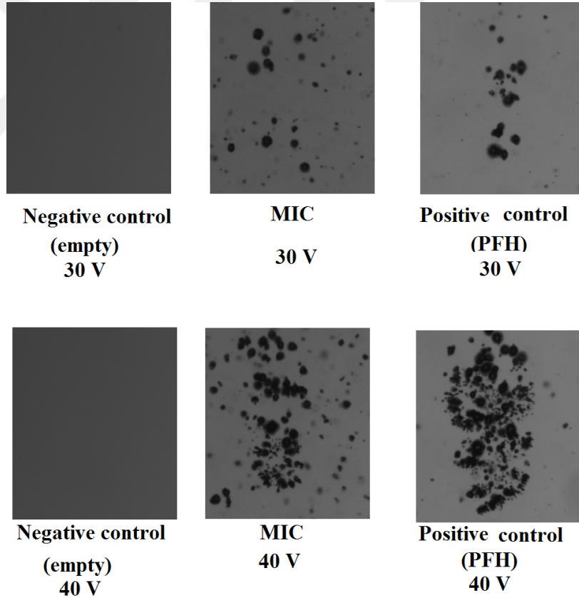
Figure 4.17: Bubble cloud was generated using MIC as historipsy agent in the agarose phantom.
