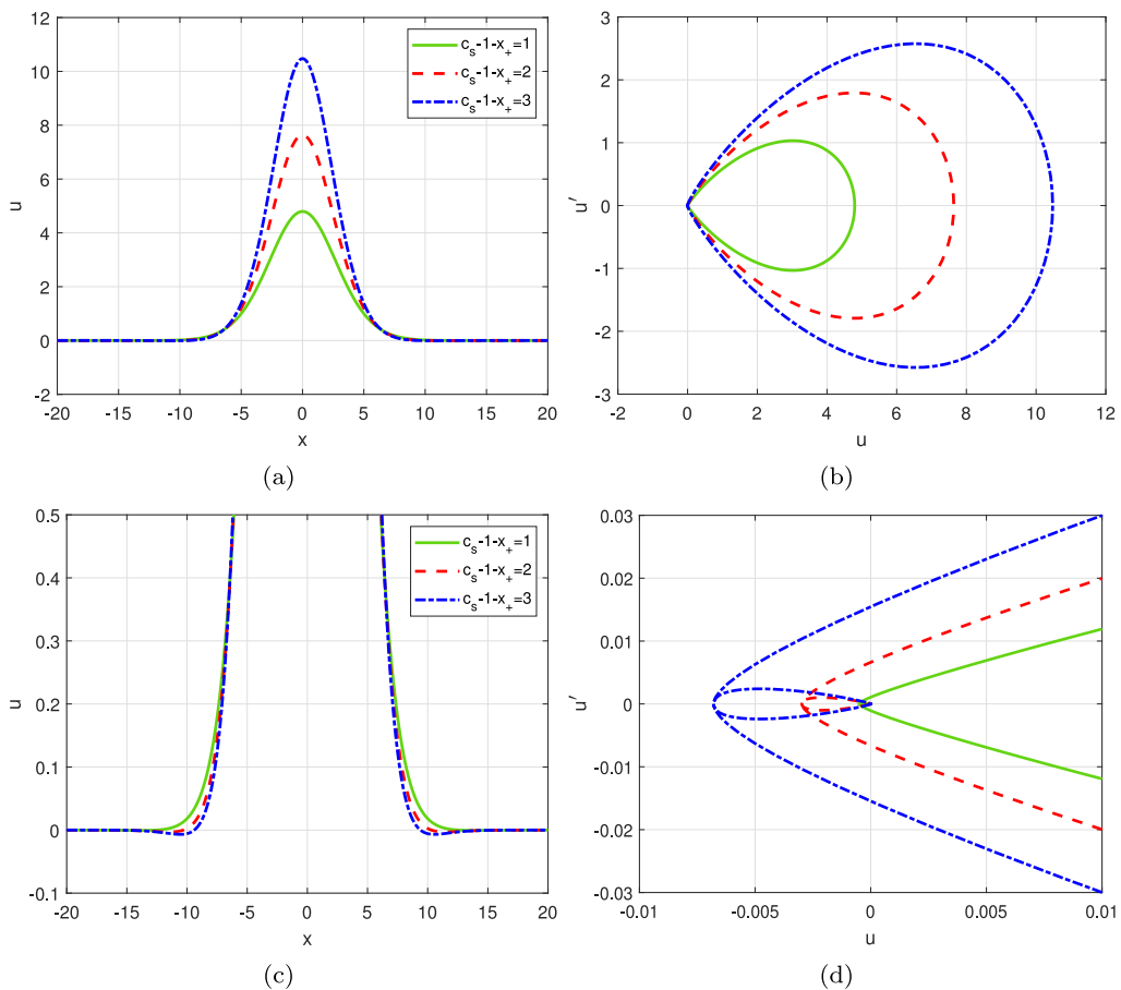
Fig. 9. Generation of NMCSW's, u profiles and phase portraits. Rosenau-RLW-Kawahara equation with \eta = 1, g(u) = u^2/2 and several speeds c_s ; (c) and (d) are magnifications of (a) and (b) resp.
