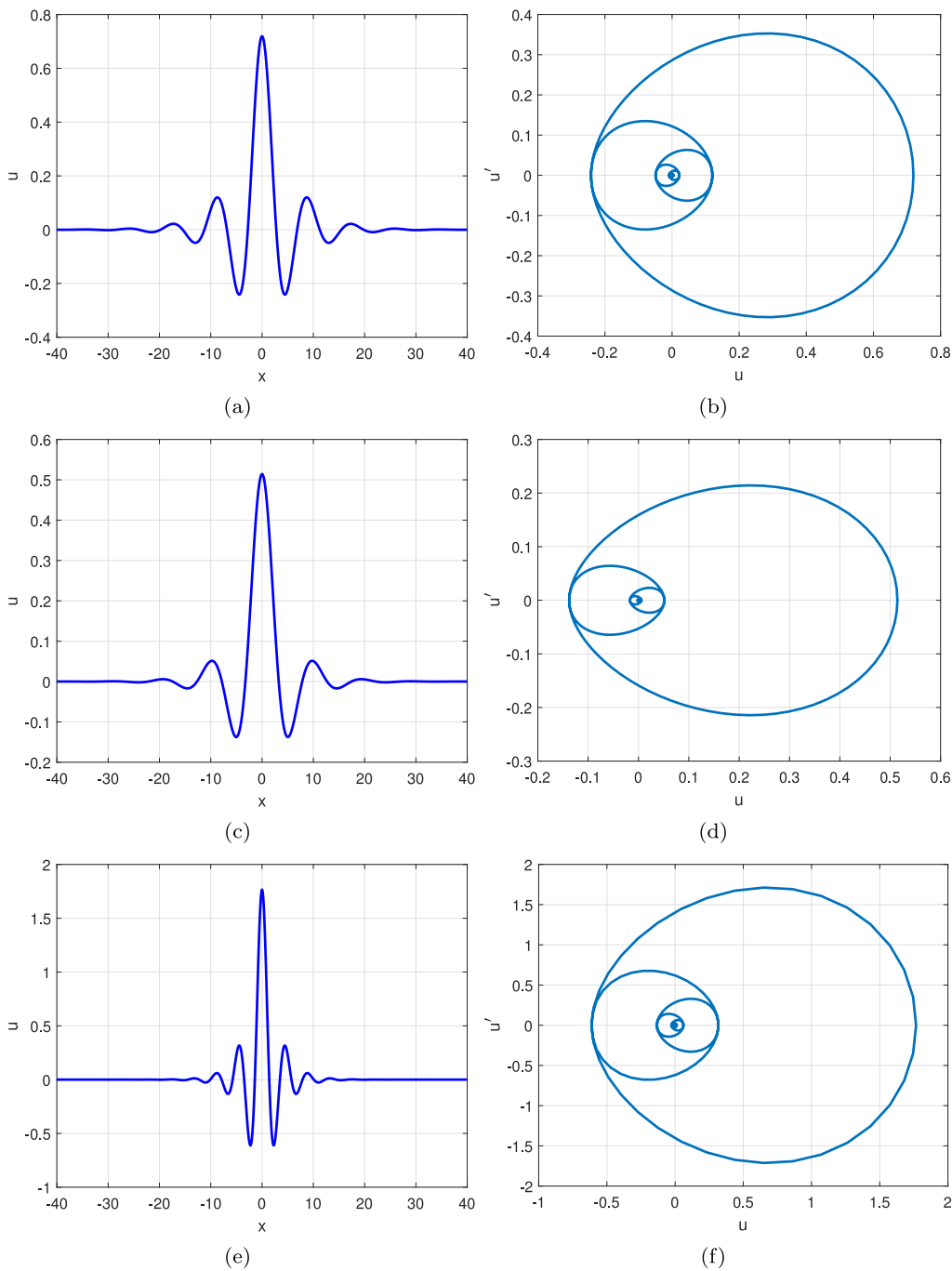
Fig. 4. Generation of nonmonotone CSWs, u profiles and phase portraits. (a), (b) Rosenau-RLW equation with \alpha = 1, \epsilon = \beta = 1, g(u) = u^2/2, c_s = 1.5 ; (c), (d) Rosenau-KdV equation with \eta = -1, \epsilon = \beta = 1, g(u) = u^2/2, c_s \approx 1.3071 ; (e), (f) Rosenau-Kawahara equation with \gamma = 2, \epsilon = \beta = 1, \eta = -1, g(u) = u^2/2, c_s \approx 2.2590 .
