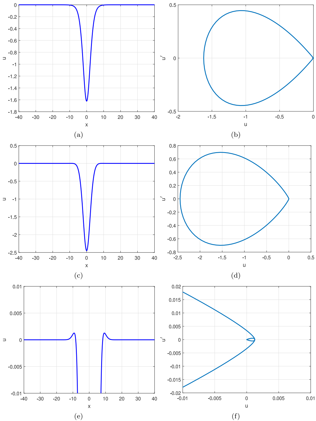
Fig. 6. Bifurcation from region 2 to region 1 close to C_3 , u profiles and phase portraits. (a), (b) Rosenau–Kawahara equation with \eta = -1, \epsilon = 1, \beta = 2, \gamma = 1, g(u) = u^2/2, c_s \approx 0.4538 ; (c), (d) Rosenau–Kawahara equation with \gamma = 1, \epsilon = 1, \beta = 2, \eta = -1, g(u) = u^2/2, c_s \approx 0.1438 ; (e) and (f) are magnifications of (c) and (d) resp.
