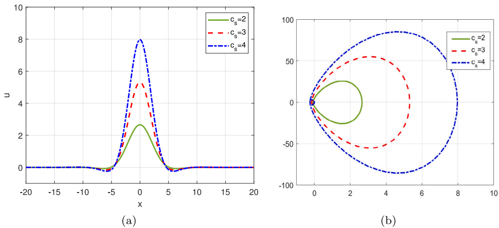
Fig. 7. Generation of nonmonotone CSW's, u profiles and phase portraits. Rosenau equation with \epsilon = \beta = 1, g(u) = u^2/2 and for several speeds c_s > \epsilon .
