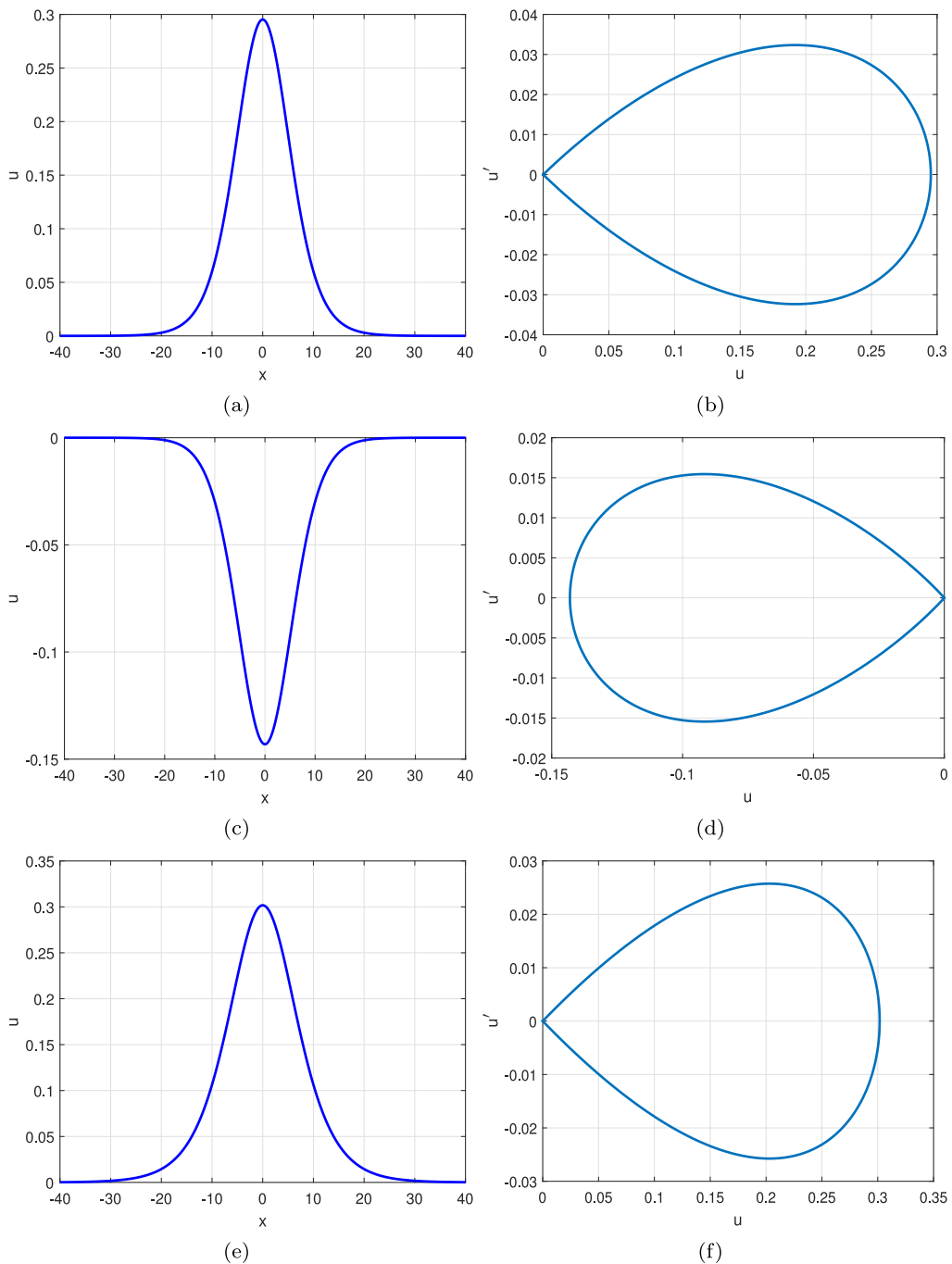
Fig. 2. CSW generation, u profiles and phase portraits. (a), (b) Rosenau-RLW equation with \alpha = -1, \epsilon = \beta = 1, g(u) = u^2/2, c_s = 1.1 ; (c), (d) Rosenau-Kawahara equation with \eta = -1/2, \epsilon = \beta = 1, \gamma = 2, g(u) = u^2/2, c_s = y_- + \epsilon + 0.01 \approx 0.951 ; (e), (f) Rosenau-RLW-Kawahara equation with \alpha = \gamma = -1, \epsilon = \beta = 1, \eta = 1, g(u) = u^2/2, c_s = z_+ + \epsilon - 0.565 \approx 1.102 . The values of y_- and z_+ are given in Tables 3 and 4 resp.
