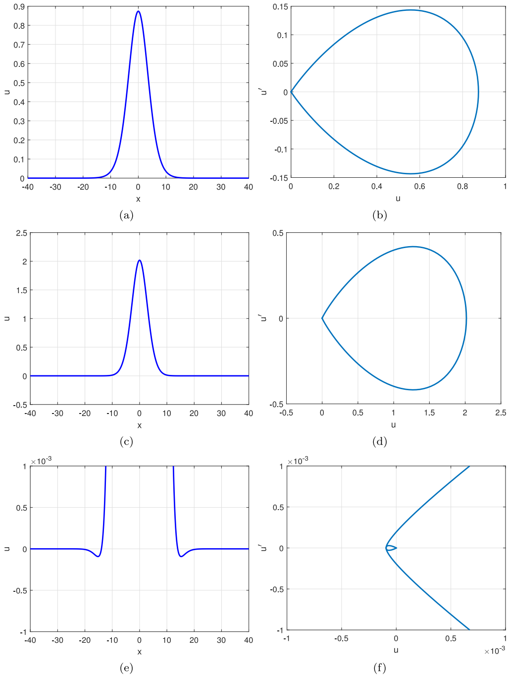
Fig. 5. Bifurcation from region 2 to region 1 close to C_3 , u profiles and phase portraits. (a), (b) Rosenau-RLW equation with \alpha = -1, \epsilon = \beta = 1, g(u) = u^2/2; c_s = 1.3 ; (c), (d) Rosenau-RLW equation with \alpha = -1, \epsilon = \beta = 1, g(u) = u^2/2; c_s = 1.7 ; (e) and (f) are magnifications of (c) and (d) resp.
