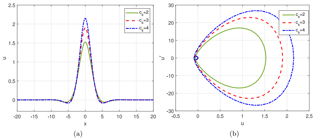
Fig. 8. Generation of nonmonotone CSW's, u profiles and phase portraits. Rosenau equation with \epsilon = \beta = 1, g(u) = u^3/3 + u^5/5 and for several speeds c_s > \epsilon .
