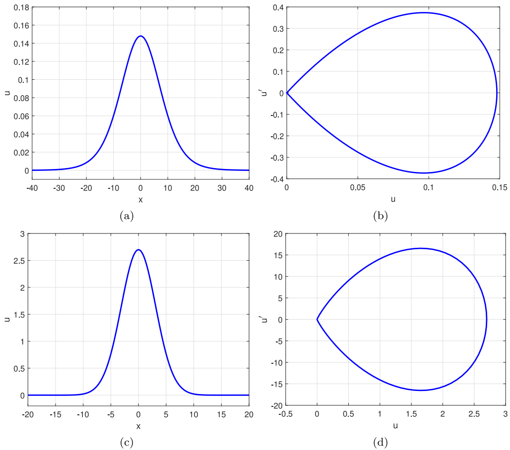
Fig. 10. Generation of CSW's, u profiles and phase portraits. Rosenau-RLW-Kawahara equation with \eta = 1 , g(u) = u^2 + u_x^2 + uu_{xx} and speeds (a), (b) c_s = 1.1 ; (c), (d) c_s = 2.9 .
