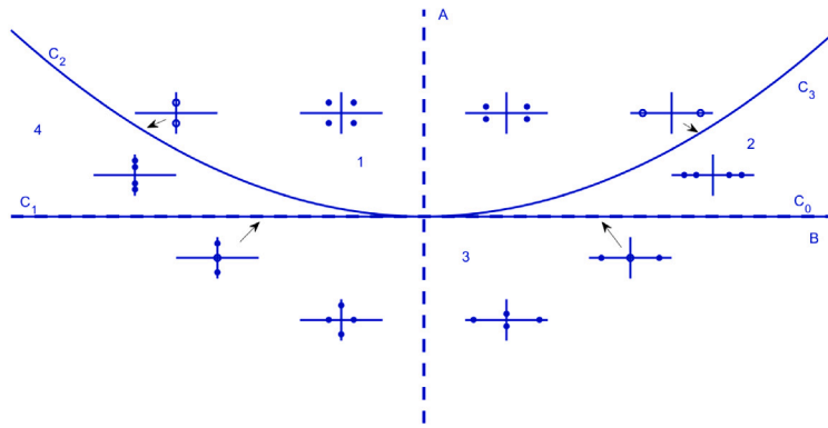
Fig. 1. Linearization at the origin of (3.1) (as in Figure 1 of [1]): Regions 1 to 4 in the (b, a) -plane, delimited by the bifurcation curves C_0 to C_3 , and schematic representation of the position in the complex plane of the roots of (3.5) for each curve and region. (Dot: simple root, larger dot: double root).
