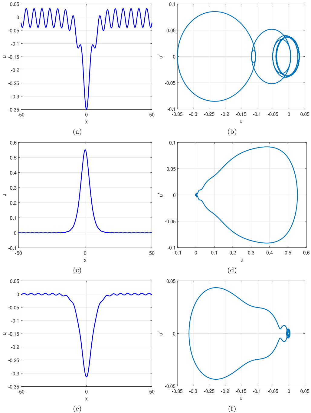
Fig. 3. GSW generation, u profiles and phase portraits. (a), (b) Rosenau-RLW equation with \alpha = 1, \epsilon = \beta = 1, g(u) = u^2/2, c_s = 0.9 ; (c), (d) Rosenau-Kawahara equation with \eta = 1, \epsilon = 0.25, \beta = 4, \gamma = 2, g(u) = u^2/2, c_s = 0.43 ; (e), (f) Rosenau-Kawahara equation with \eta = -1, \epsilon = 1, \beta = 2, \gamma = 1, g(u) = u^2/2, c_s = 0.9 .
